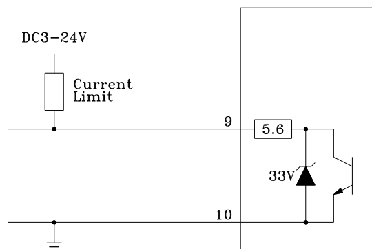
<Output Circuit>
